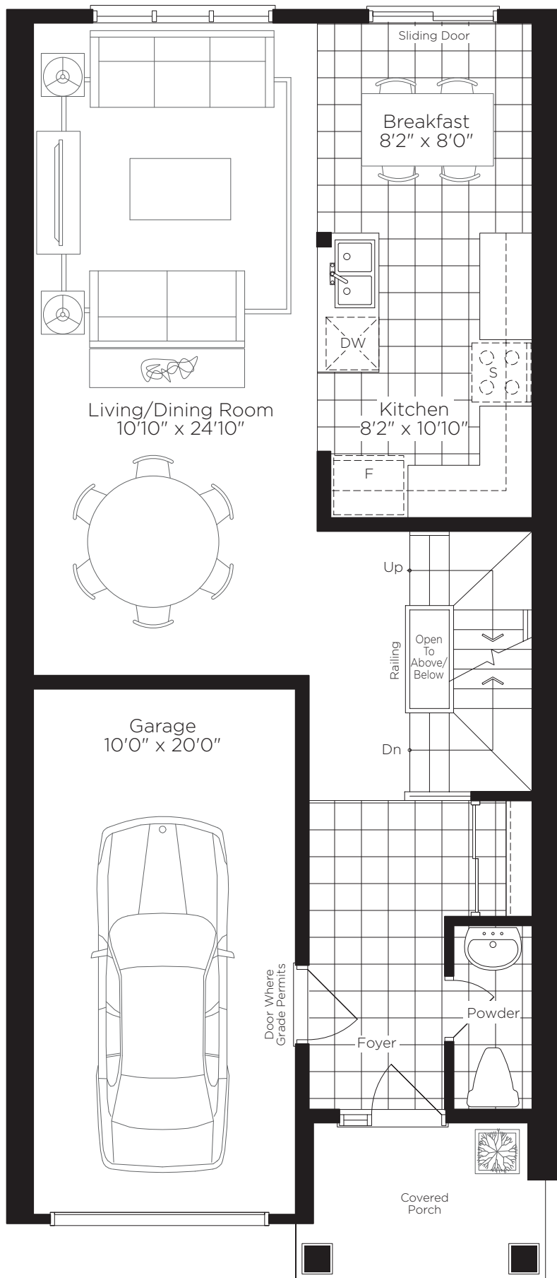
Ground Floor Elev. A & B
