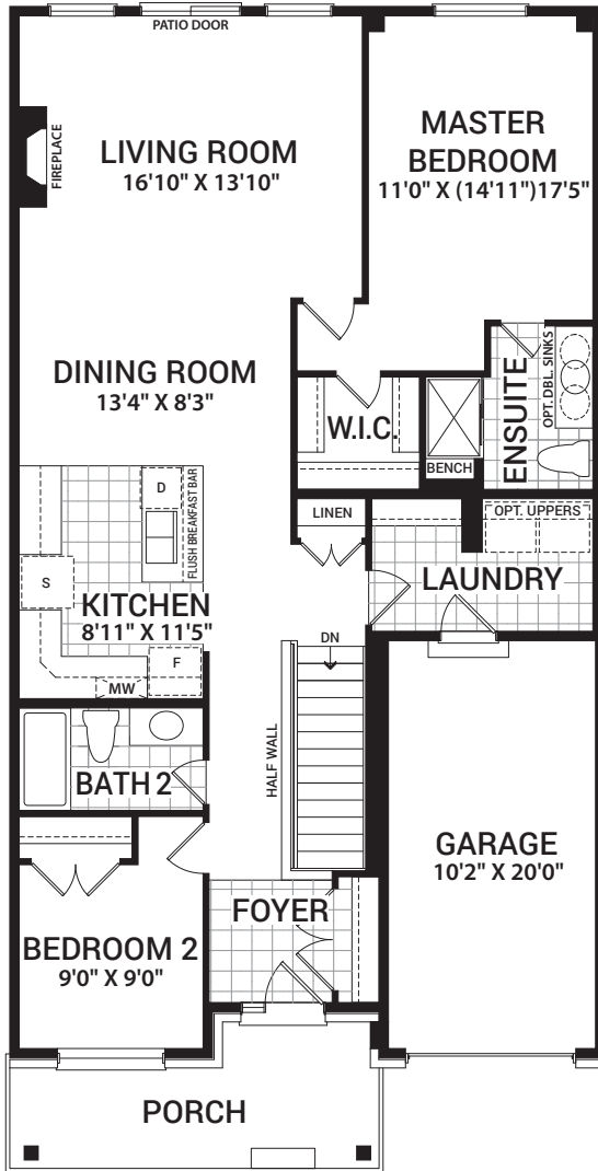
MAIN FLOOR PLAN A
