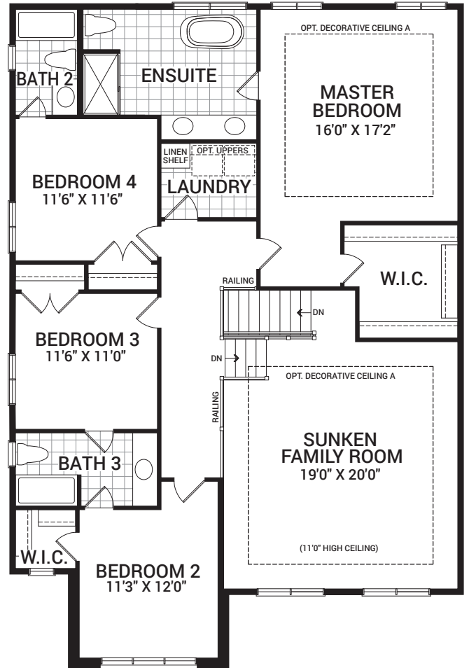
SECOND FLOOR PLAN A
