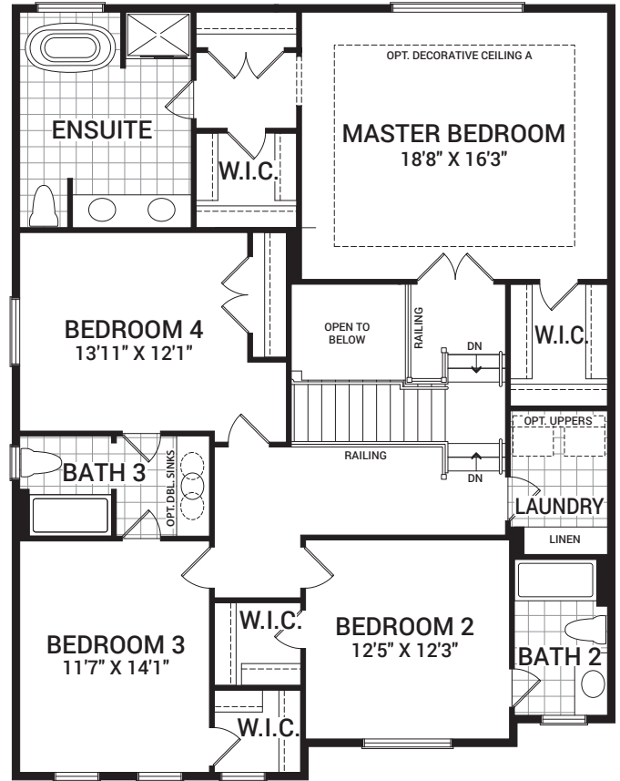
SECOND FLOOR PLAN A
