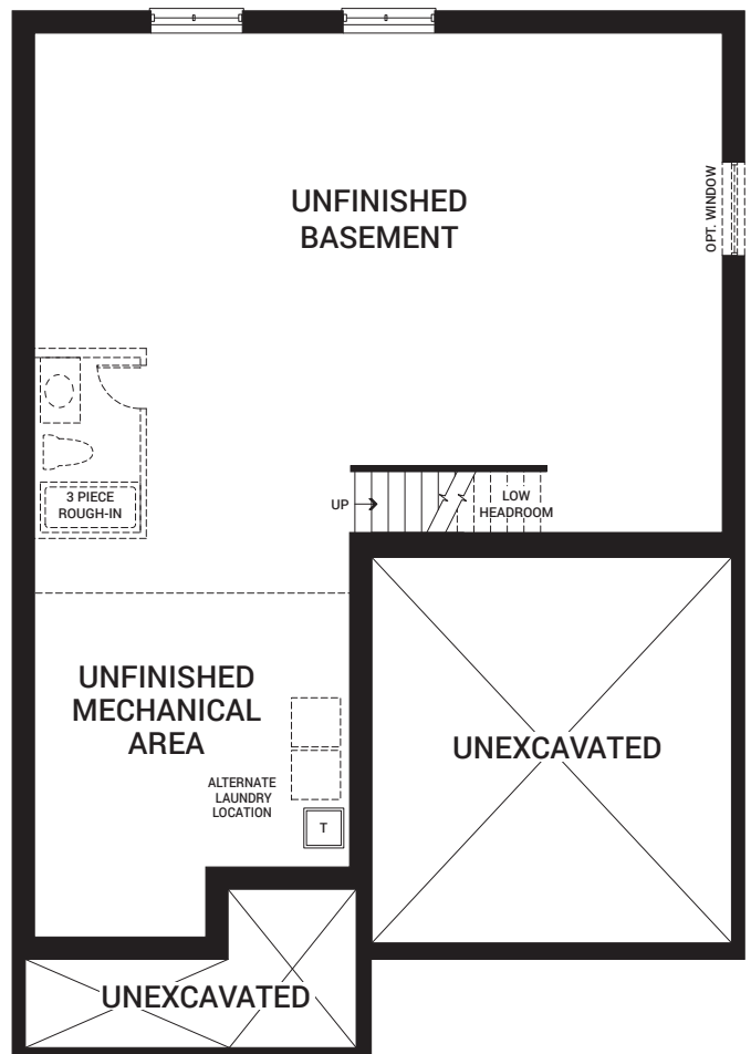
BASEMENT FLOOR PLAN A
