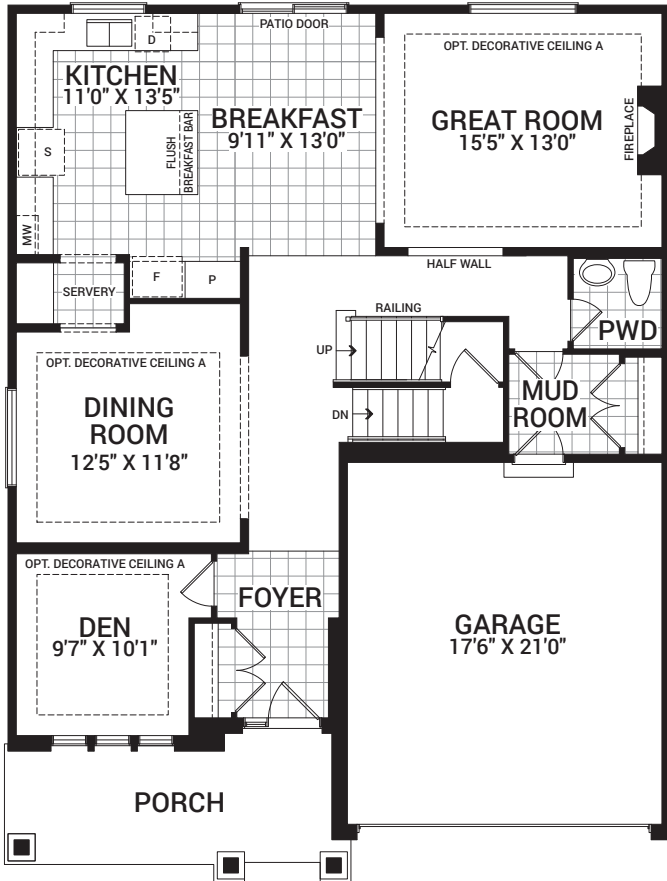
MAIN FLOOR PLAN A
