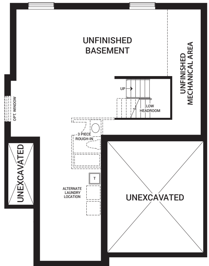
BASEMENT PLAN A & B
