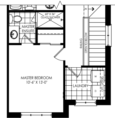
ELEVATION B OPT. LAUNDRY WITH 4 BEDROOM ON GROUND FLOOR
