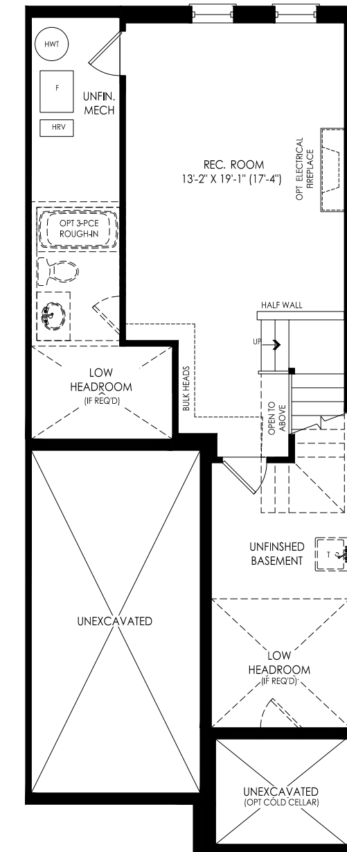
ELEVATION AA
