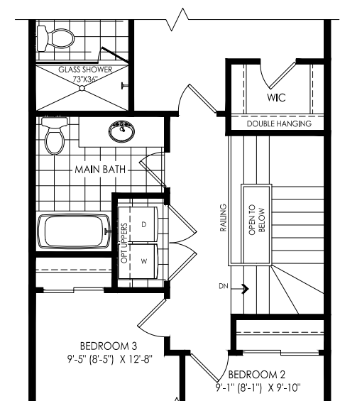
ELEVATION AC & BC FLEX PLAN WITH LAUNDRY
