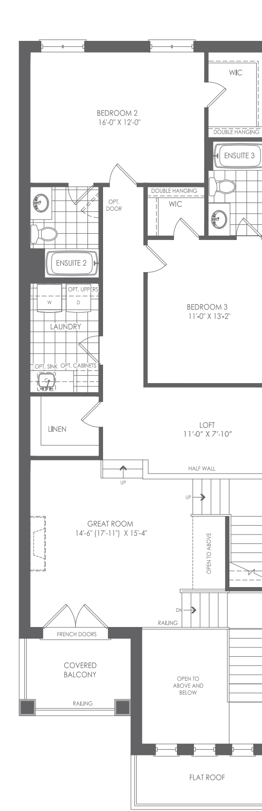
OPTIONAL SECOND FLOOR ELEV. A
