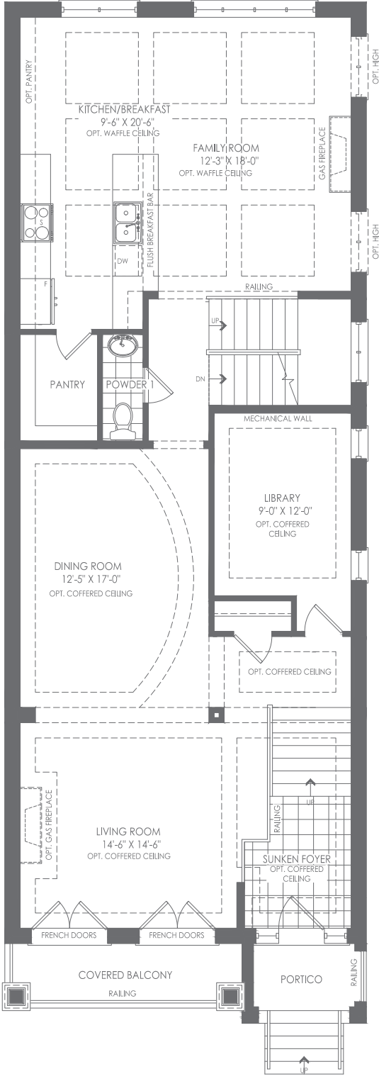
SECOND FLOOR ELEV. A (MAIN LIVING/KITCHEN LEVEL)
