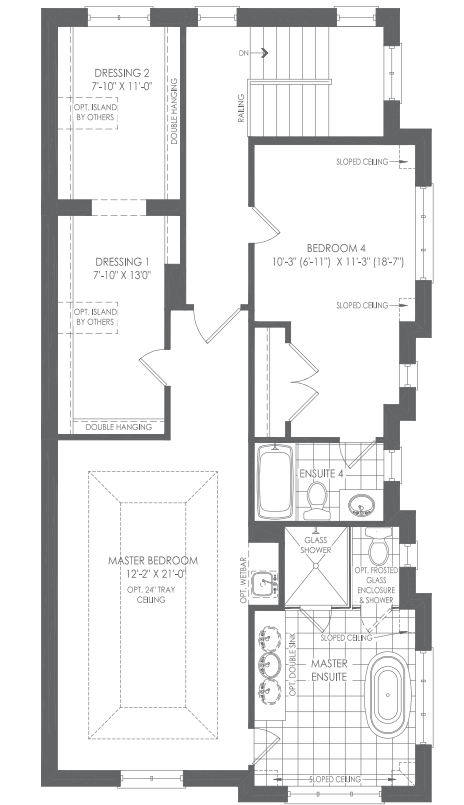
THIRD FLOOR ELEV. A
