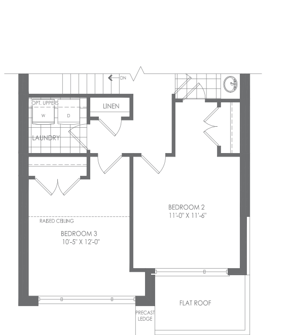
PARTIAL STANDARD AND OPTIONAL THIRD FLOOR ELEV. B
