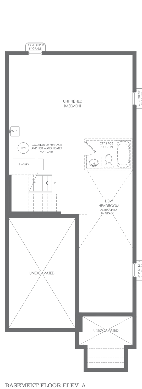
BASEMENT FLOOR ELEV. A
