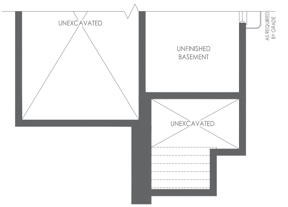
PARTIAL BASEMENT FLOOR ELEV. B
