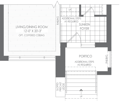
PARTIAL SECOND FLOOR ELEV. B
