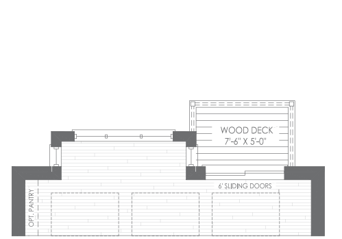
OPTIONAL DECK CONDITION - FOR INTERNAL LOTS ONLY
