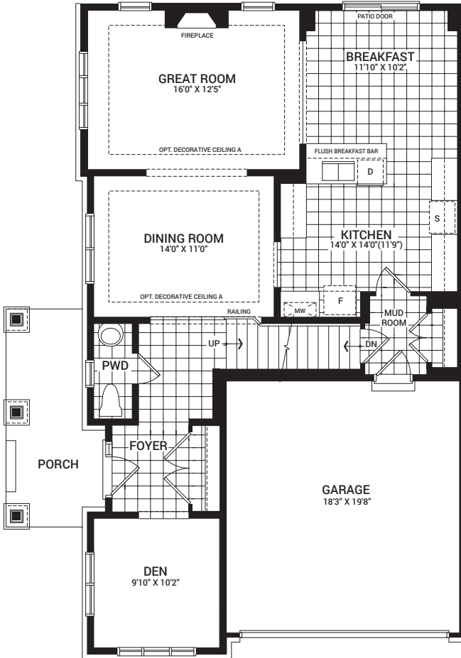
MAIN FLOOR PLAN A
