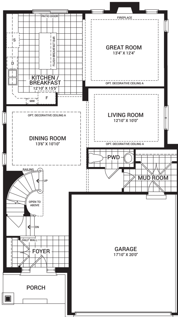
MAIN FLOOR PLAN A
