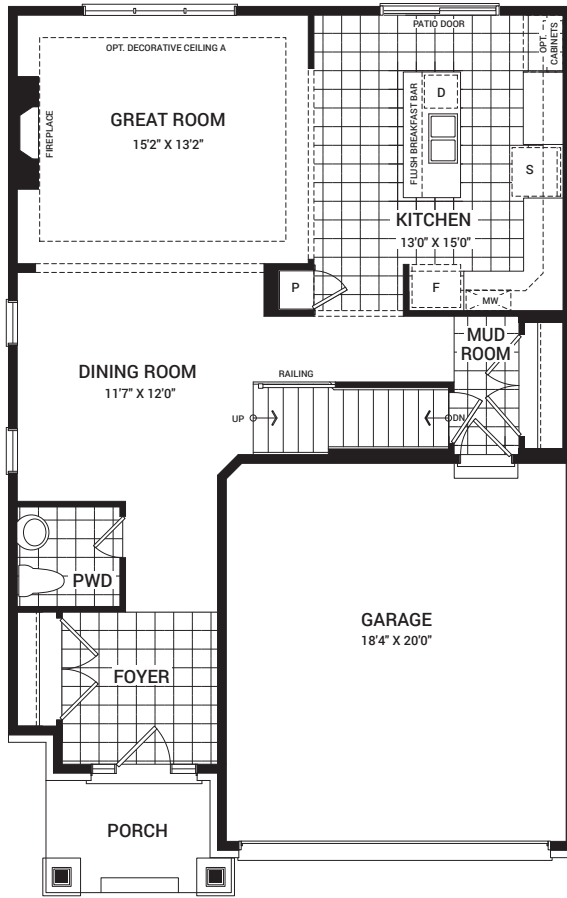
MAIN FLOOR PLAN A
