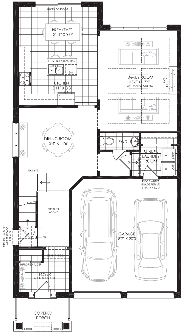
GROUND FLOOR PLAN ELEV. 'A'
