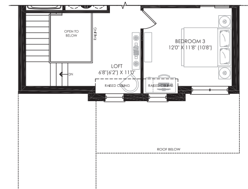
PARTIAL SECOND FLOOR PLAN ELEV. 'D'
