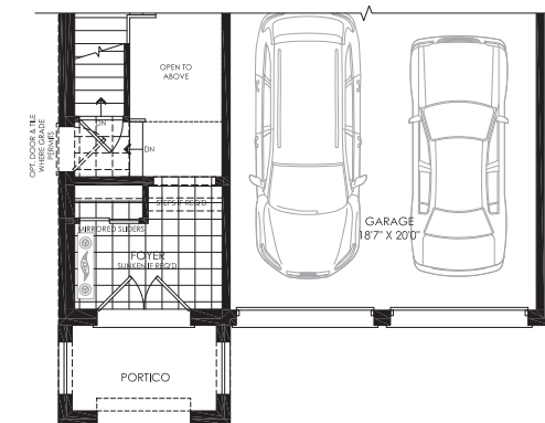
PARTIAL GROUND FLOOR PLAN ELEV. 'D'
