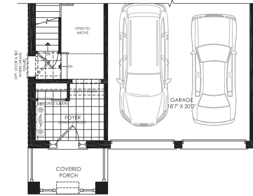
PARTIAL GROUND FLOOR PLAN ELEV. 'B'
