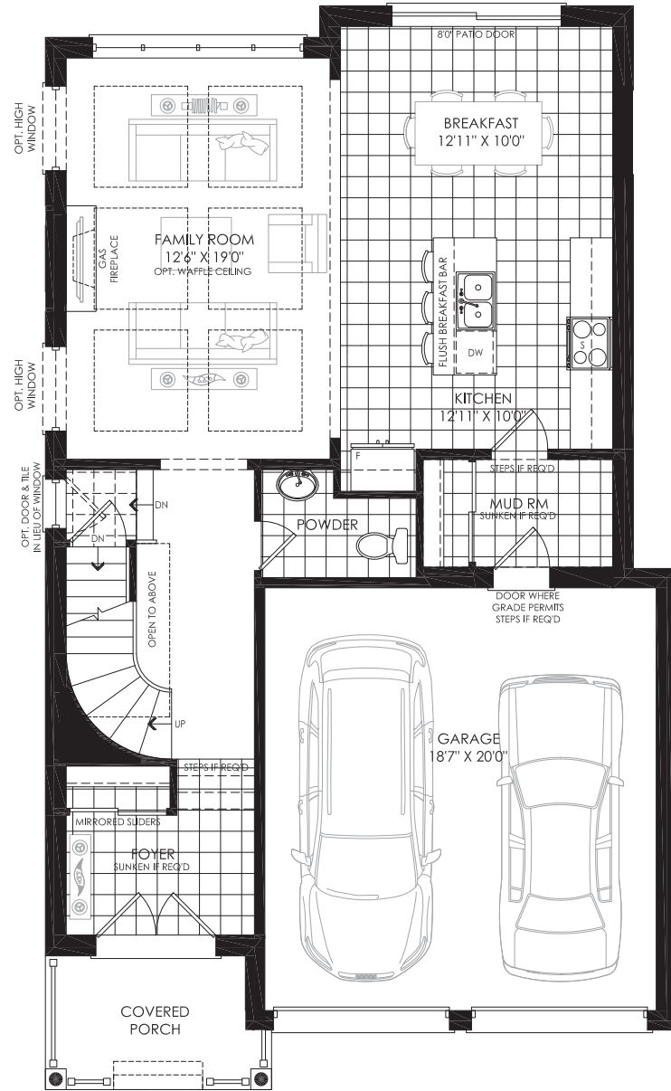
GROUND FLOOR PLAN ELEV. 'A'
