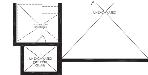
PARTIAL BASEMENT PLAN ELEV. 'B'
