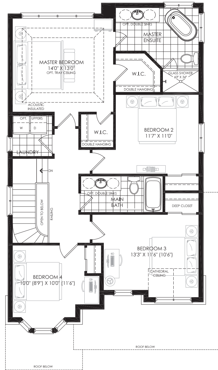
SECOND FLOOR PLAN ELEV. 'A'
