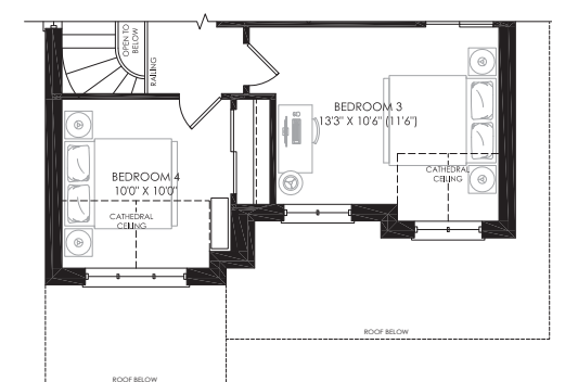
PARTIAL SECOND FLOOR PLAN ELEV. 'D'
