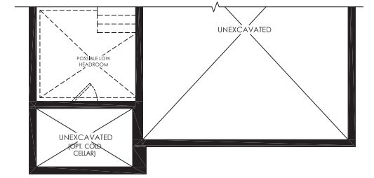
PARTIAL BASEMENT PLAN ELEV. 'D'
