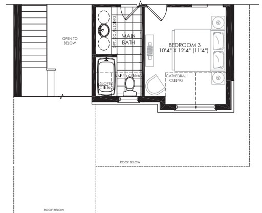
PARTIAL SECOND FLOOR PLAN ELEV. 'B'
