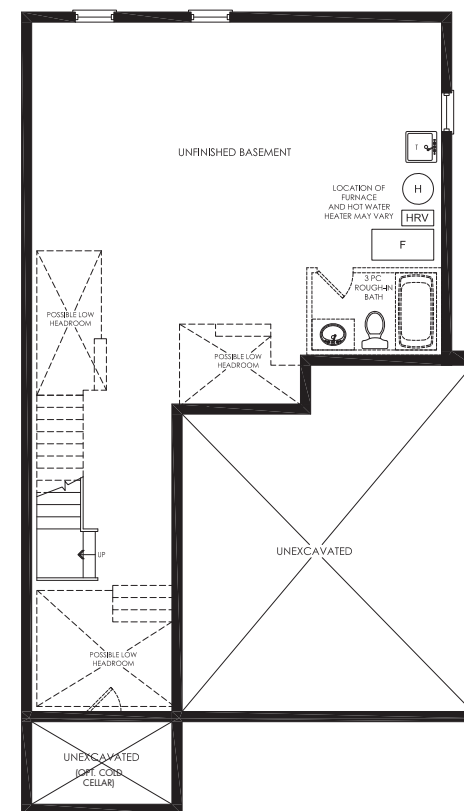
BASEMENT PLAN ELEV. 'A', 'B' & 'D'
