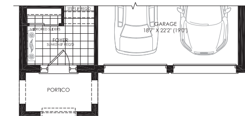
PARTIAL GROUND FLOOR PLAN ELEV. 'D'
