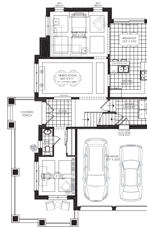
GROUND FLOOR PLAN ELEV. 'D'
