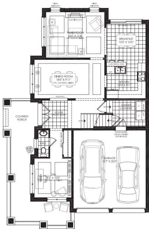
GROUND FLOOR PLAN ELEV. 'A'
