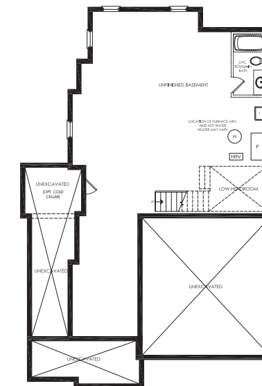
BASEMENT PLAN ELEV. 'D'
