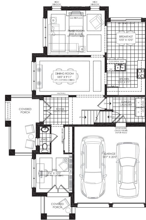
GROUND FLOOR PLAN ELEV. 'B'
