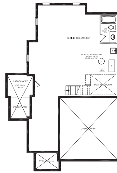
BASEMENT PLAN ELEV. 'B'
