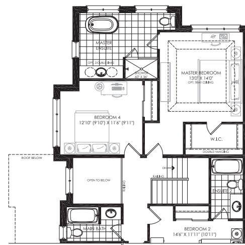
PARTIAL SECOND FLOOR PLAN FLEX PLAN WITH 3 BATHS ELEV. 'B'
