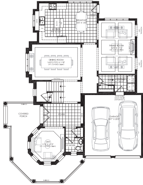
GROUND FLOOR PLAN ELEV. 'A'
