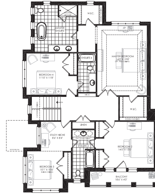
SECOND FLOOR PLAN ELEV. 'B'
