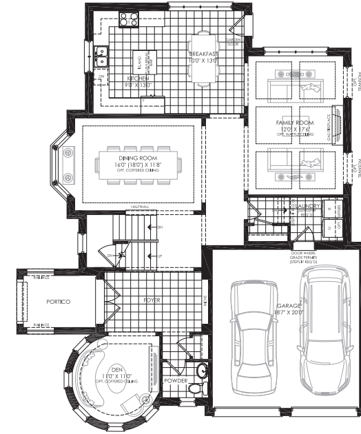
GROUND FLOOR PLAN ELEV. 'D'
