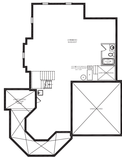
BASEMENT PLAN ELEV. 'A'
