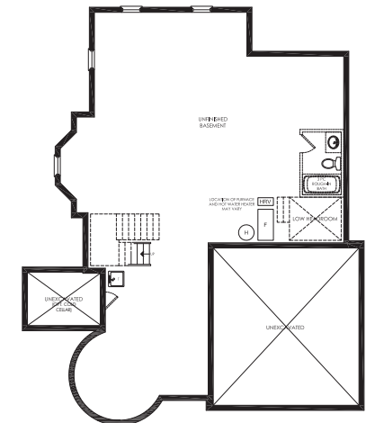
BASEMENT PLAN ELEV. 'D'
