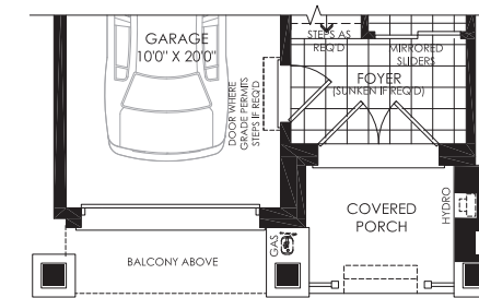
PARTIAL GROUND FLOOR PLAN ELEV. BC
