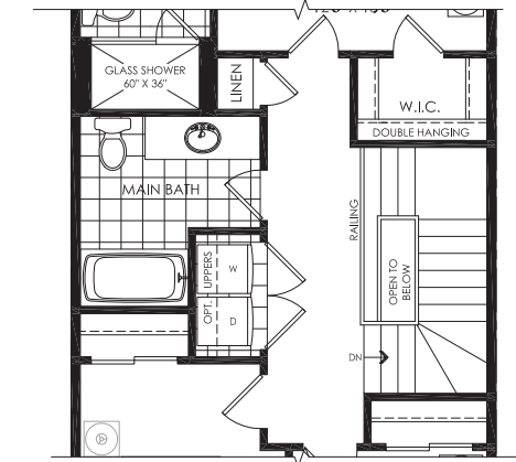
PARTIAL SECOND FLOOR FLEX PLAN W/ LAUNDRY ELEV. AA & BC
