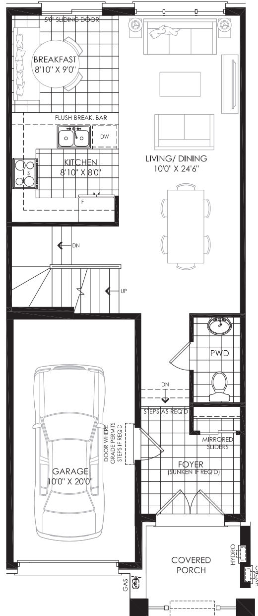
GROUND FLOOR PLAN ELEV. AA
