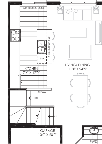
PARTIAL GROUND FLOOR FLEX PLAN ELEV. AA & BB
