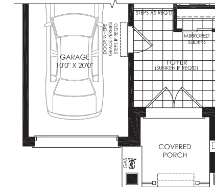
PARTIAL GROUND FLOOR PLAN ELEV. BB
