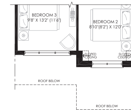
PARTIAL SECOND FLOOR PLAN ELEV. BB
