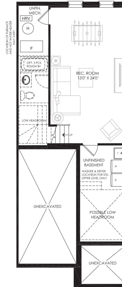
BASEMENT PLAN ELEV. AA
