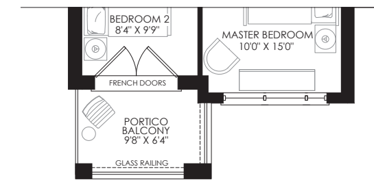
PARTIAL THIRD FLOOR & THIRD FLOOR FLEX PLAN ELEV. 'C'
