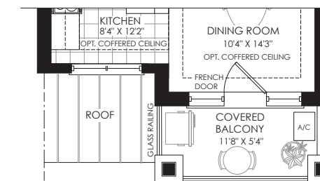
PARTIAL SECOND FLOOR PLAN ELEV. 'F'
