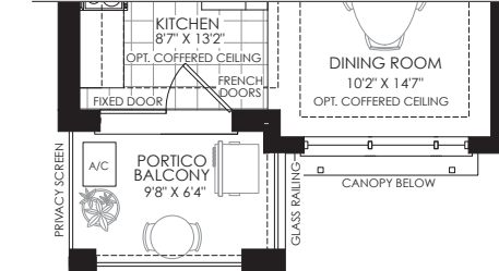
PARTIAL SECOND FLOOR PLAN ELEV. 'C'
