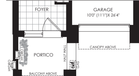
PARTIAL GROUND FLOOR PLAN ELEV. 'C'
