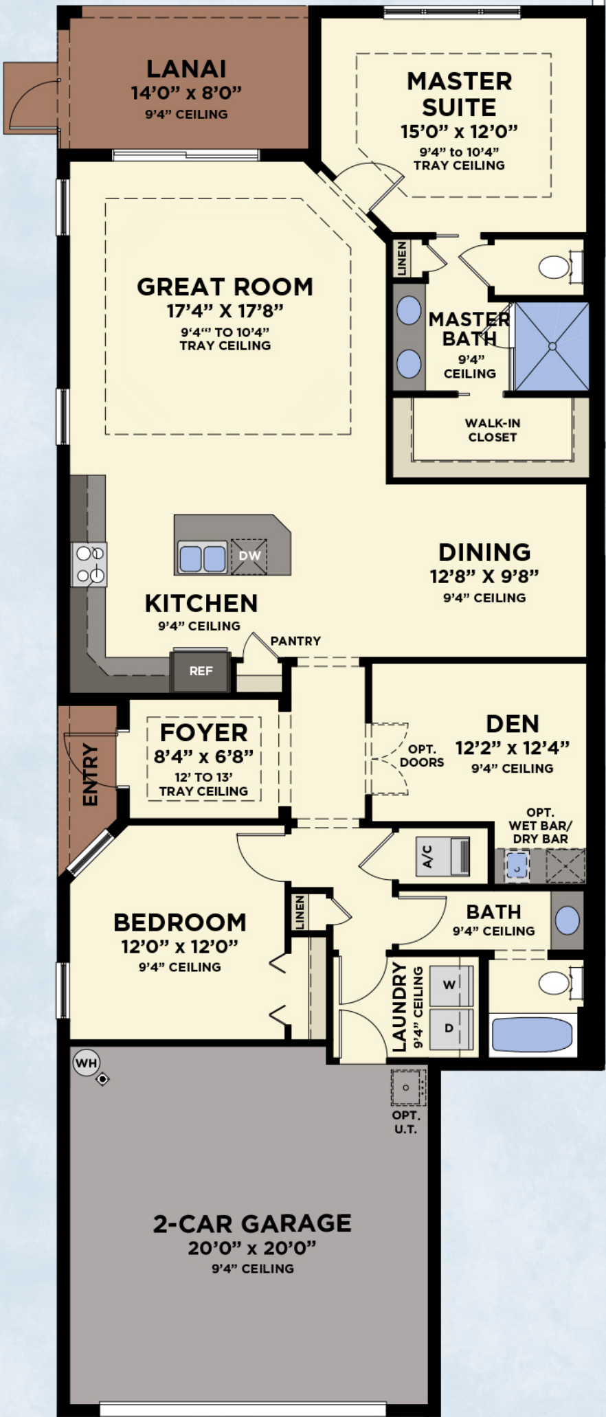
FLOOR PLAN
