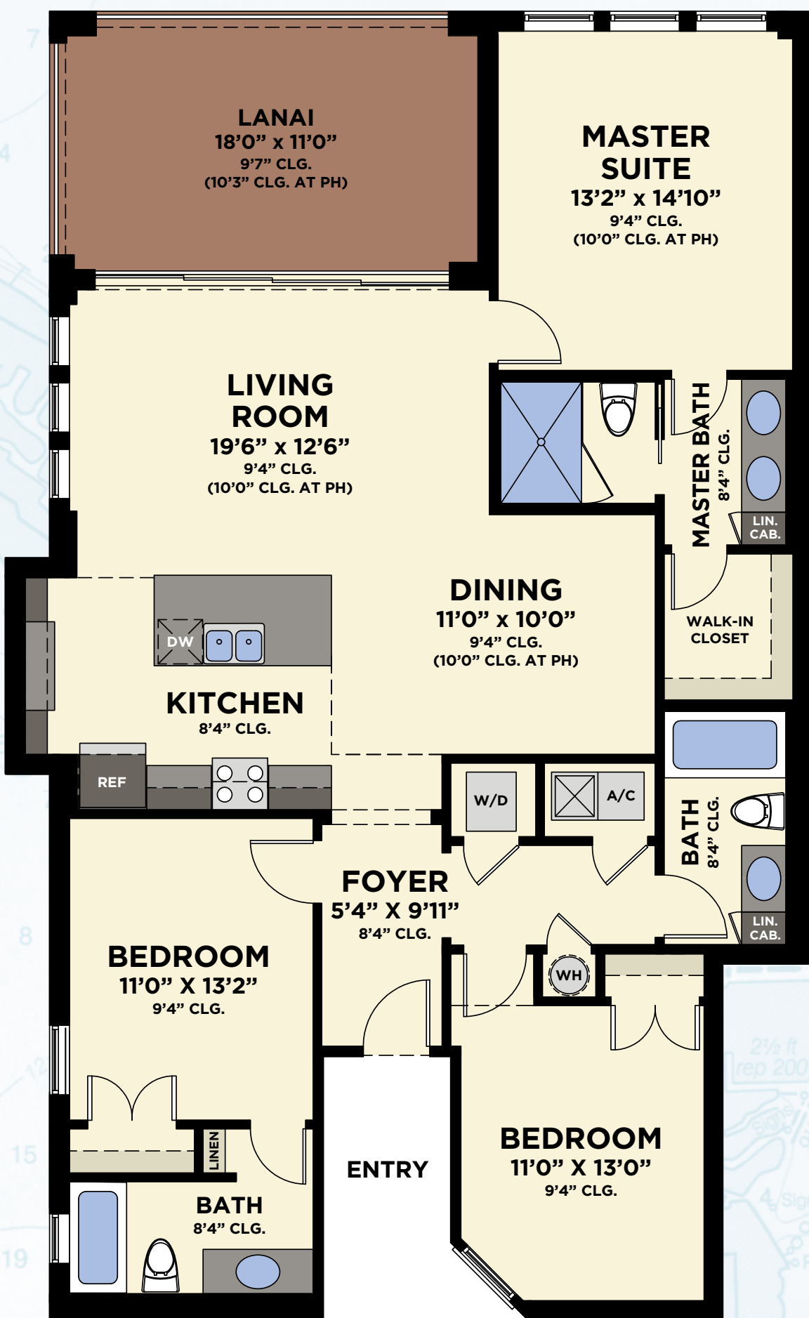
FLOORPLAN
