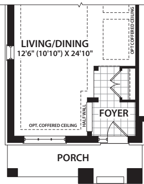
FLEX PLAN FOR LIVING/DINING ROOM
