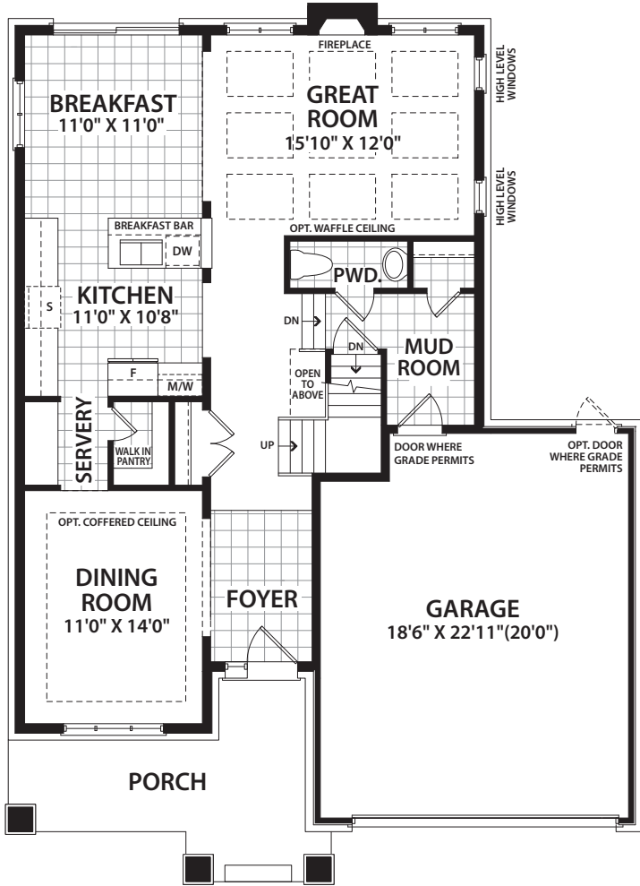
MAIN FLOOR PLAN ELEV. A
