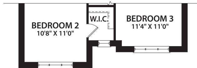
SECOND FLOOR PLAN ELEV. B
