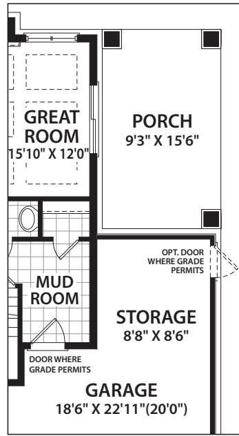
MAIN FLOOR PLAN FLEX GARAGE STORAGE
