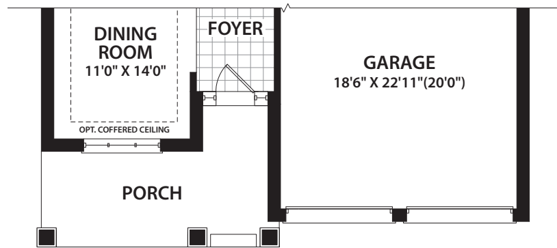
MAIN FLOOR PLAN ELEV. B
