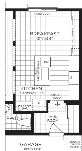
Main Floor - Flex (Relocated Dishwasher)
