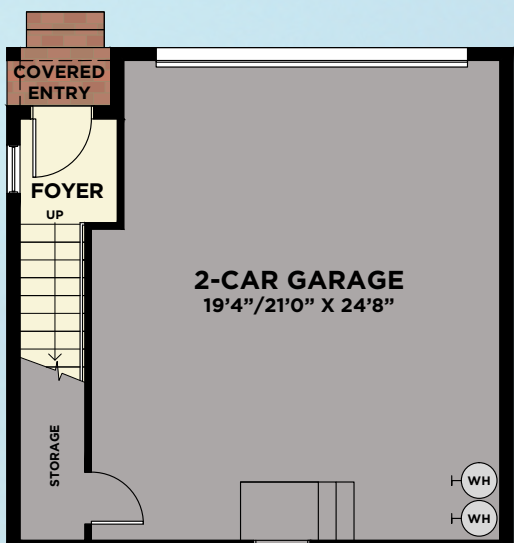
LOWER FLOOR
