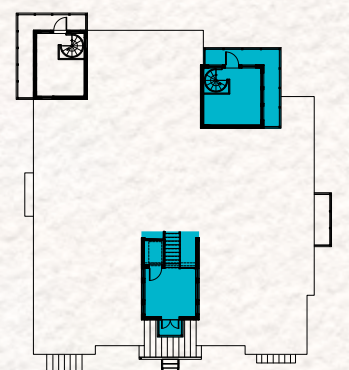
Level 3
