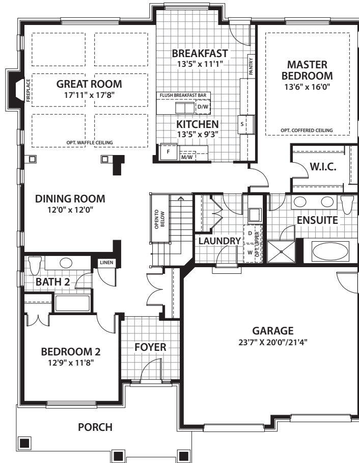
MAIN FLOOR PLAN ELEVATION A
