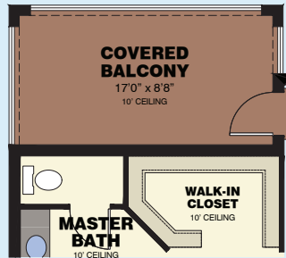
AVAILABLE BALCONY VARIATION
