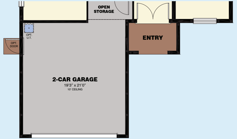
FIRST FLOOR PLAN ELEVATION 'B' VARIATION
