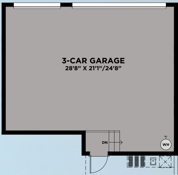
AVAILABLE 3-CAR GARAGE (731 SQ. FT.)
