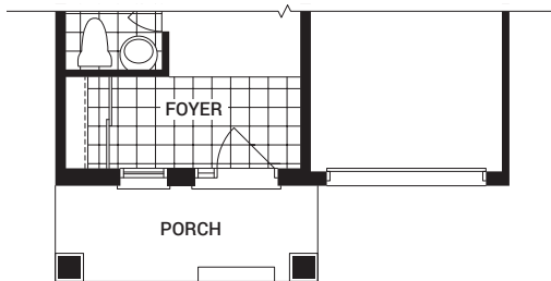
MAIN FLOOR PLAN 'B'
