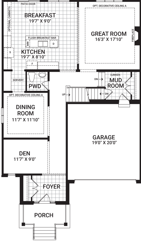
MAIN FLOOR PLAN A
