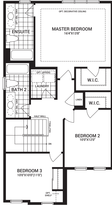
SECOND FLOOR PLAN A
