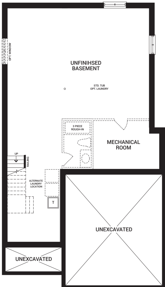
BASEMENT FLOOR PLAN ELEV. A, B & C
