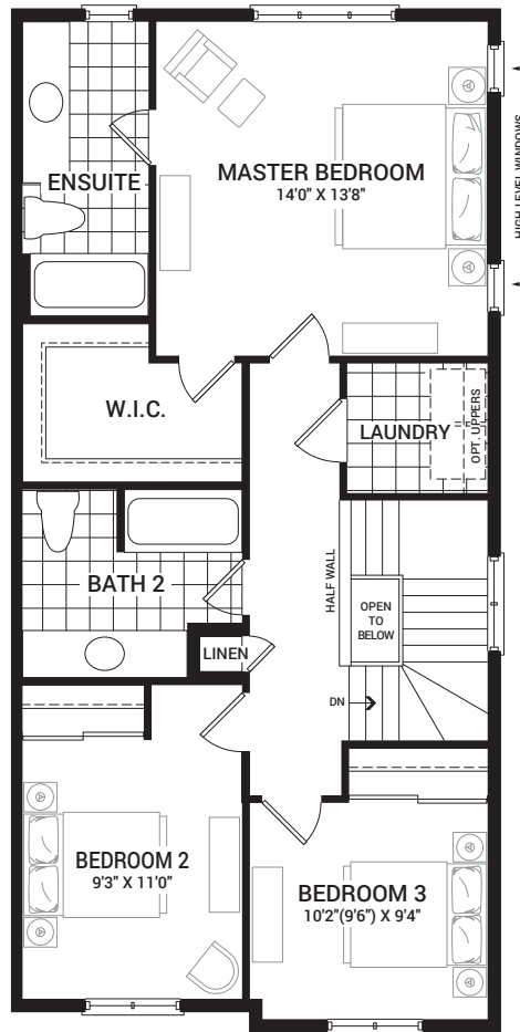
SECOND FLOOR PLAN A (COLONIAL)
