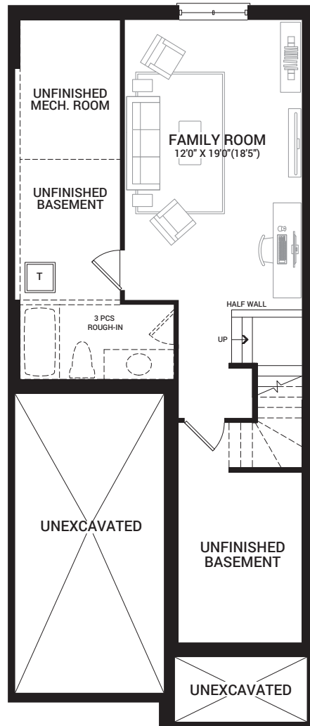
BASEMENT FLOOR PLAN A & B
