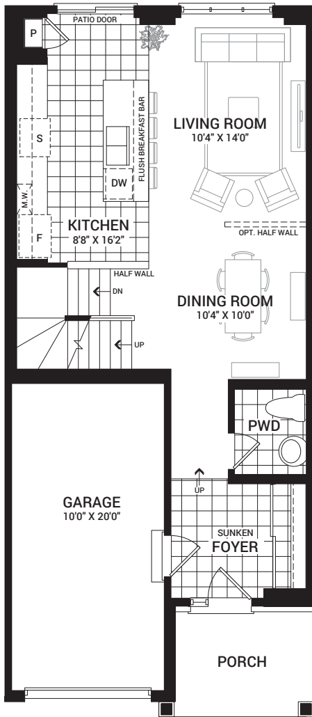
MAIN FLOOR PLAN A (COLONIAL)
