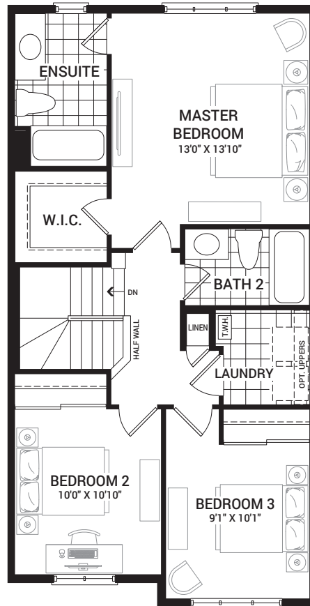
SECOND FLOOR PLAN A (COLONIAL)
