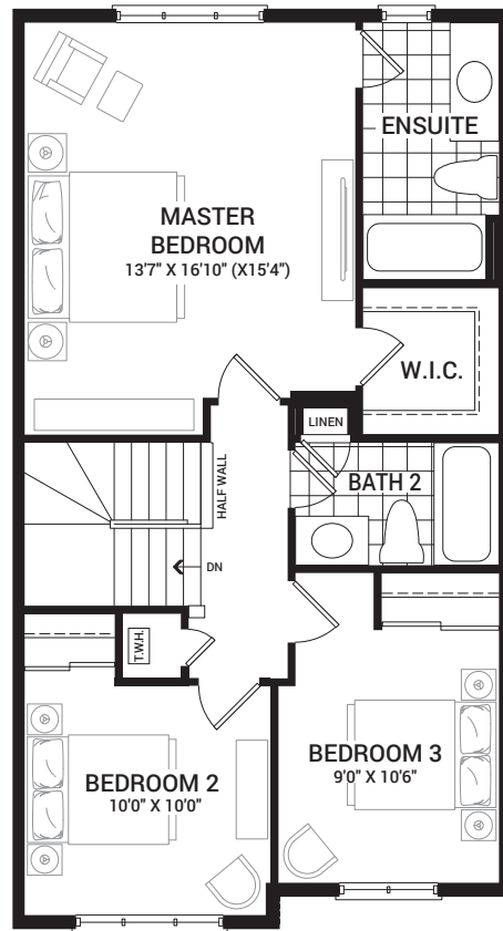
SECOND FLOOR PLAN A (COLONIAL)
