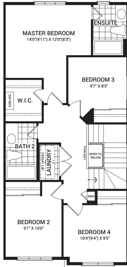
SECOND FLOOR PLAN (PRAIRIE B)
