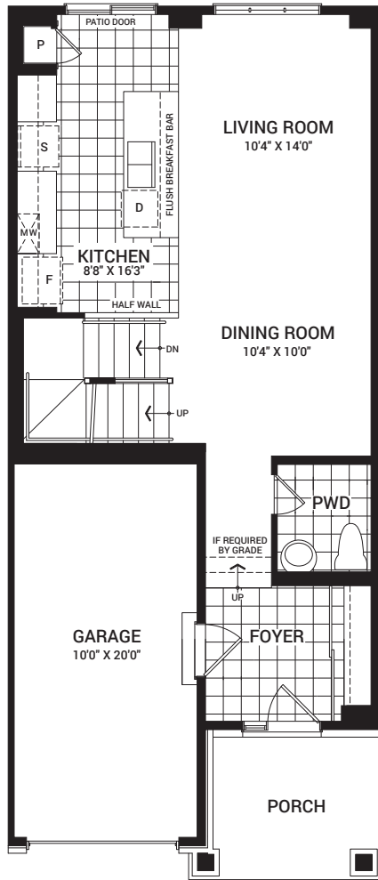
MAIN FLOOR PLAN (PRAIRIE B)
