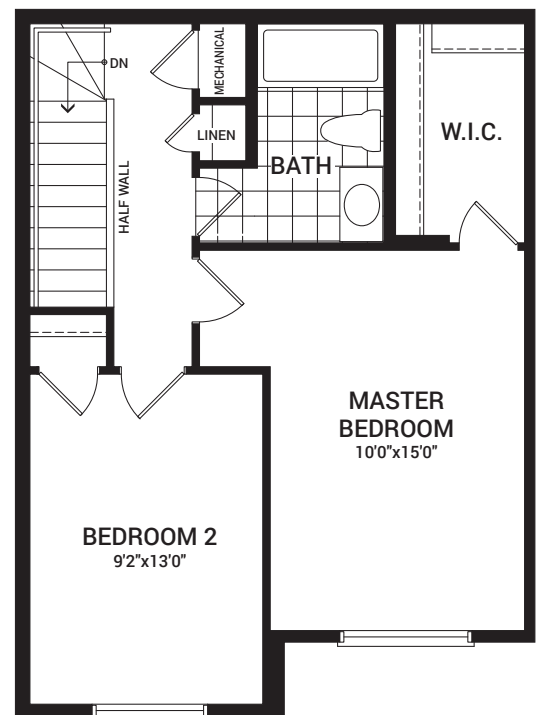
END UNIT THIRD FLOOR PLAN
