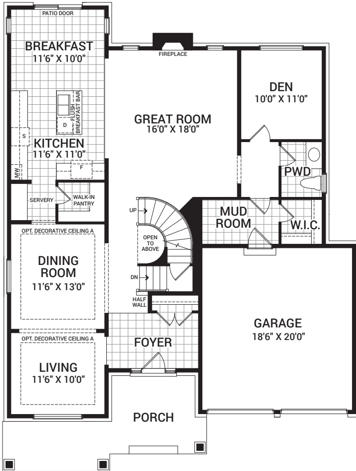
MAIN FLOOR PLAN A
