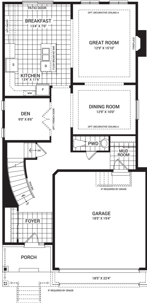
MAIN FLOOR PLAN A
