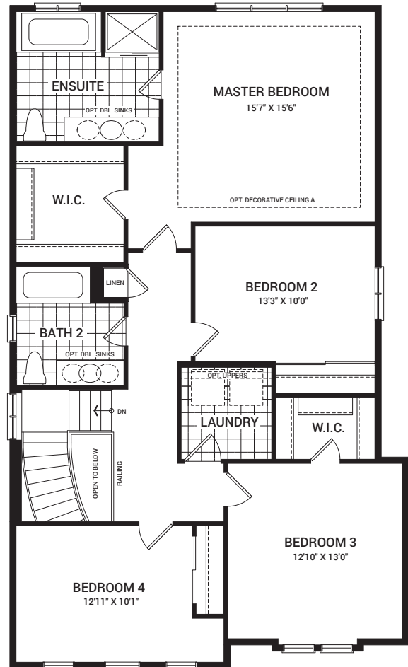
SECOND FLOOR PLAN A
