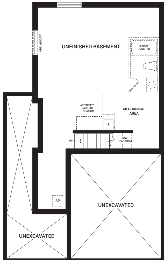
BASEMENT FLOOR PLAN A
