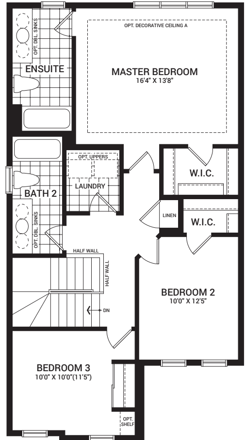
SECOND FLOOR PLAN A
