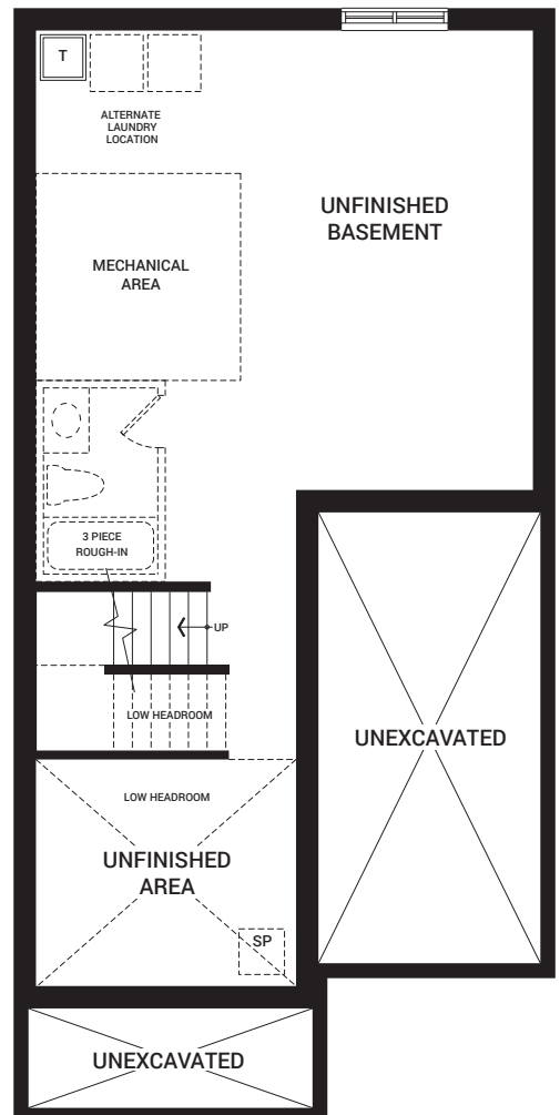
BASEMENT FLOOR PLAN A
