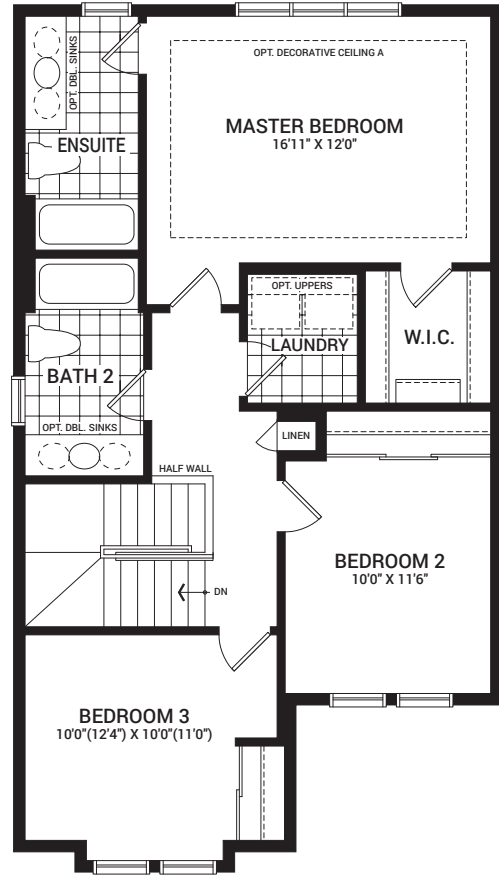
SECOND FLOOR PLAN A
