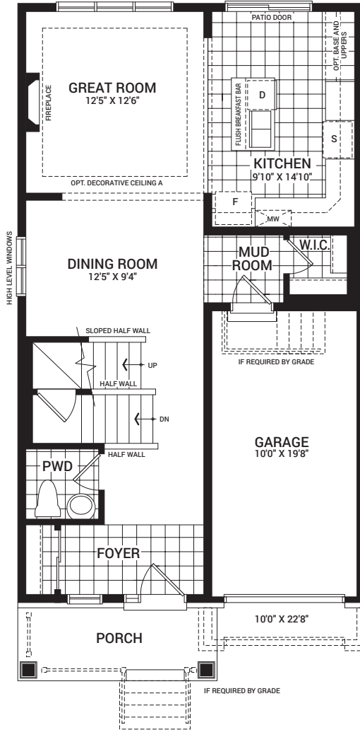
MAIN FLOOR PLAN A
